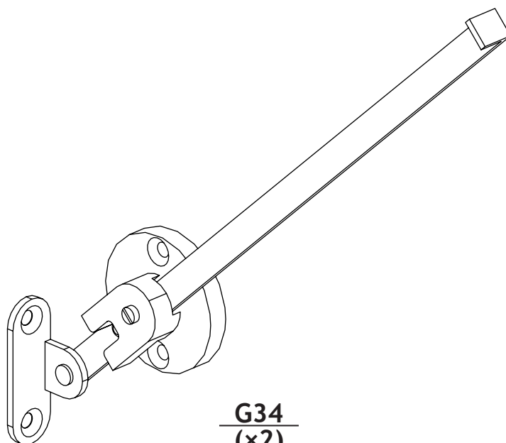
B113 (×4) L=96mm
