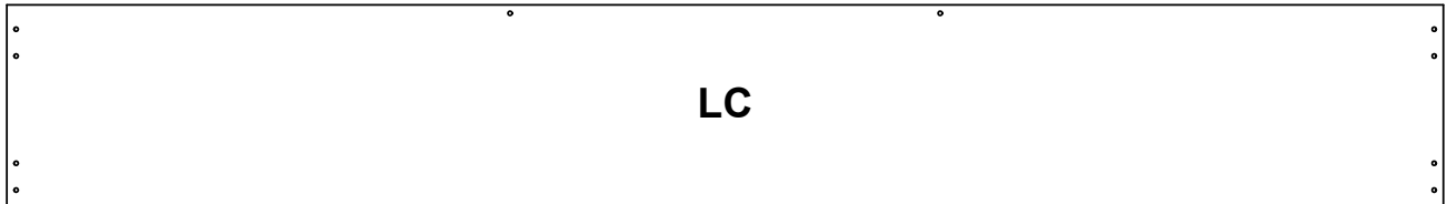
1710x240x22mm
