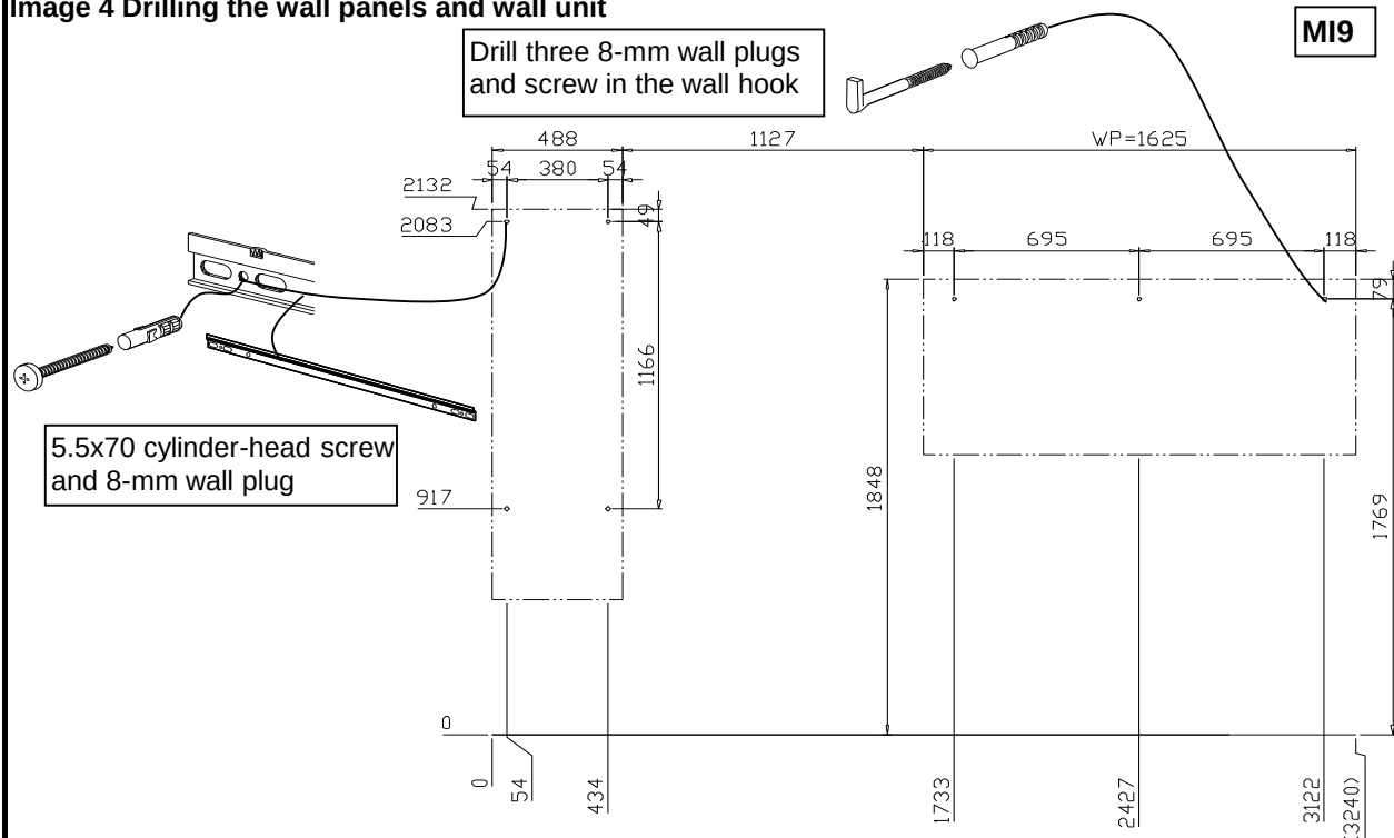
Image 4 Drilling the wall panels and wall unit
