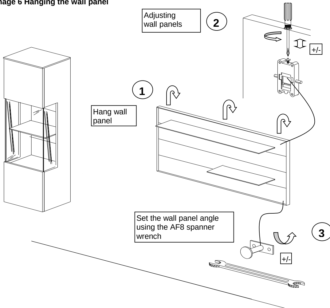
Image 6 Hanging the wall panel
