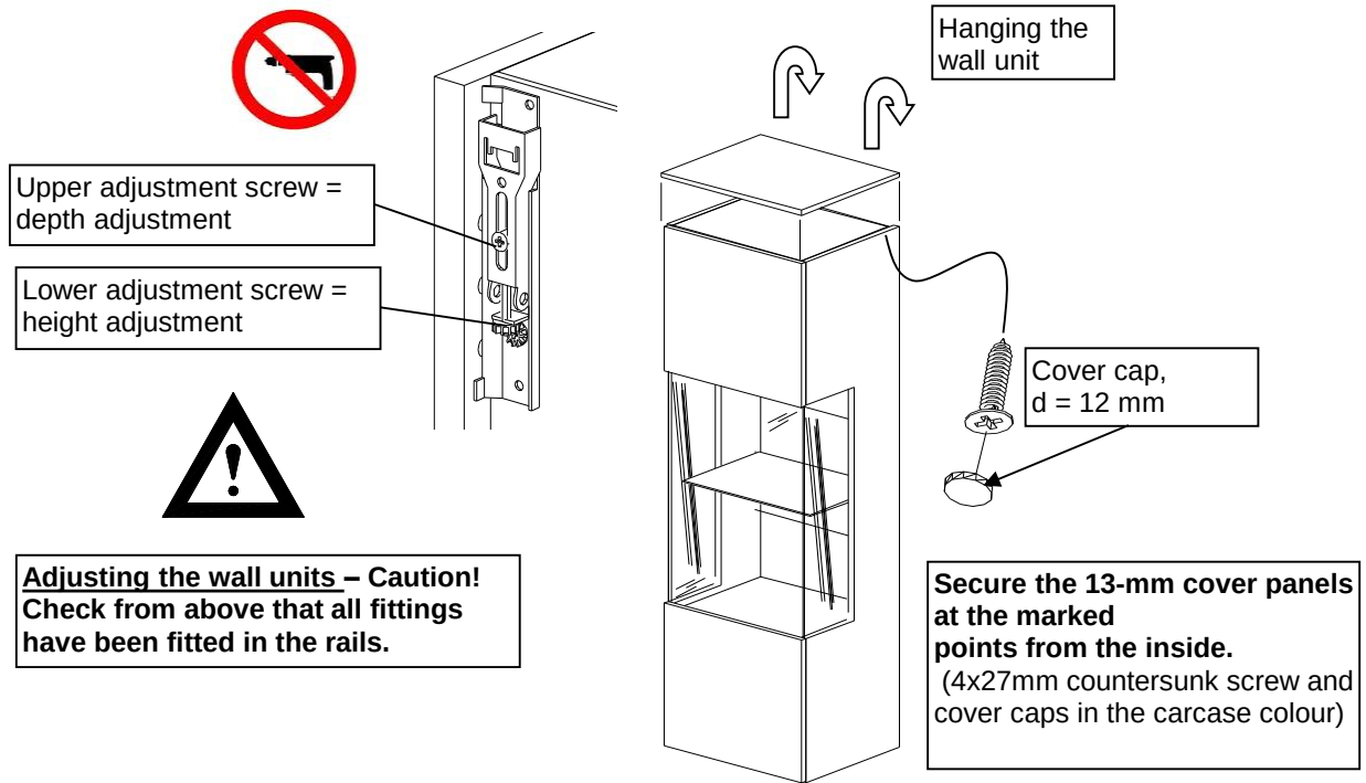
Image 5 Hanging the wall unit, securing the cover panel
