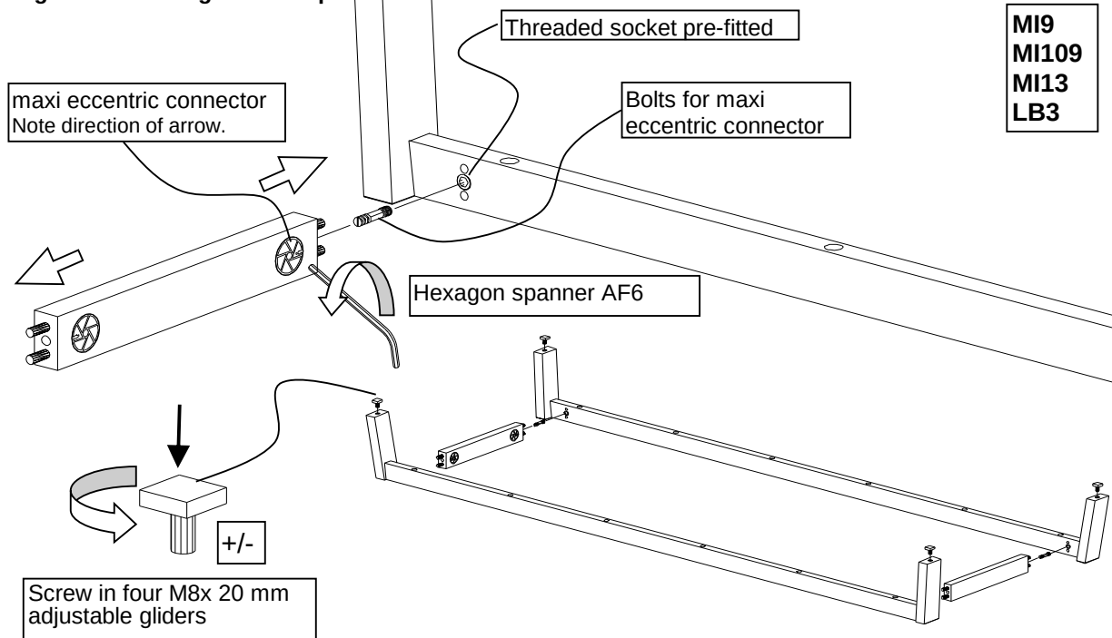
Image 8 Securing the base panel
