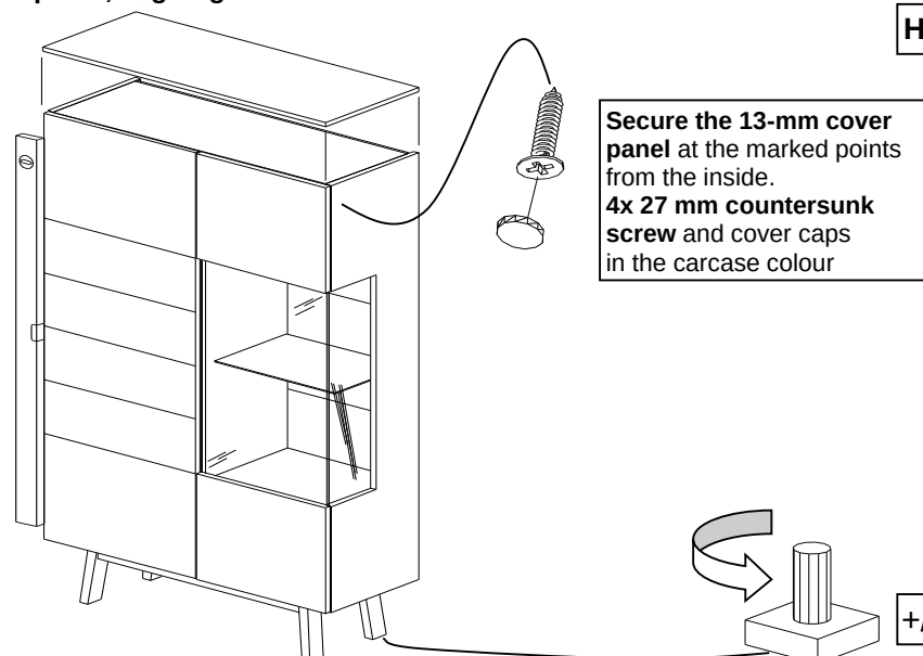
Image 16 Fitting the cover panel, aligning the cabinet
