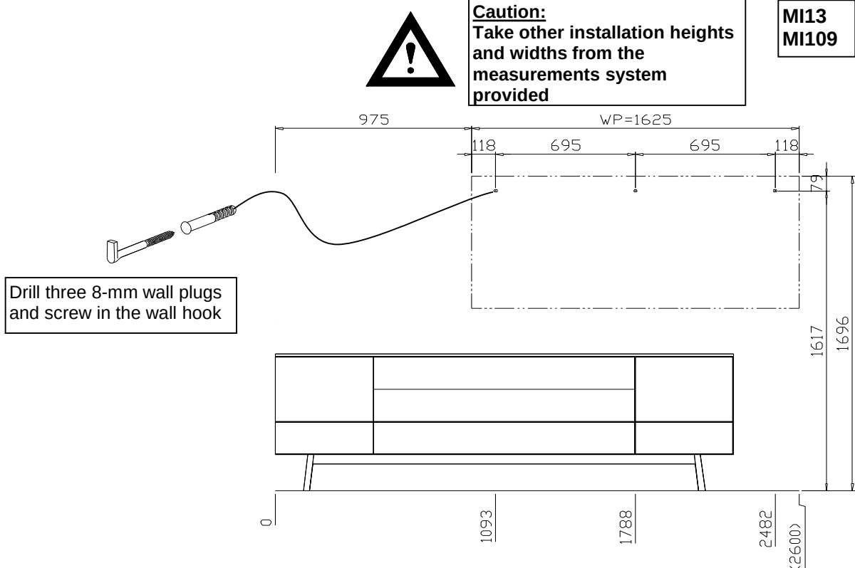
Image 11 Drilling the wall panels and wall unit
