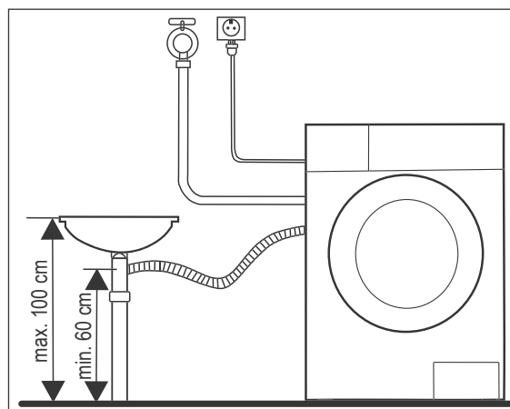
Variant 1: Connect outlet hose directly to a siphon.
