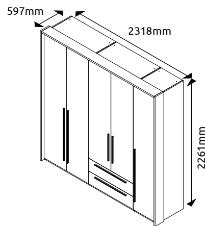
P52B/PN LWH - 2318x597x2261
